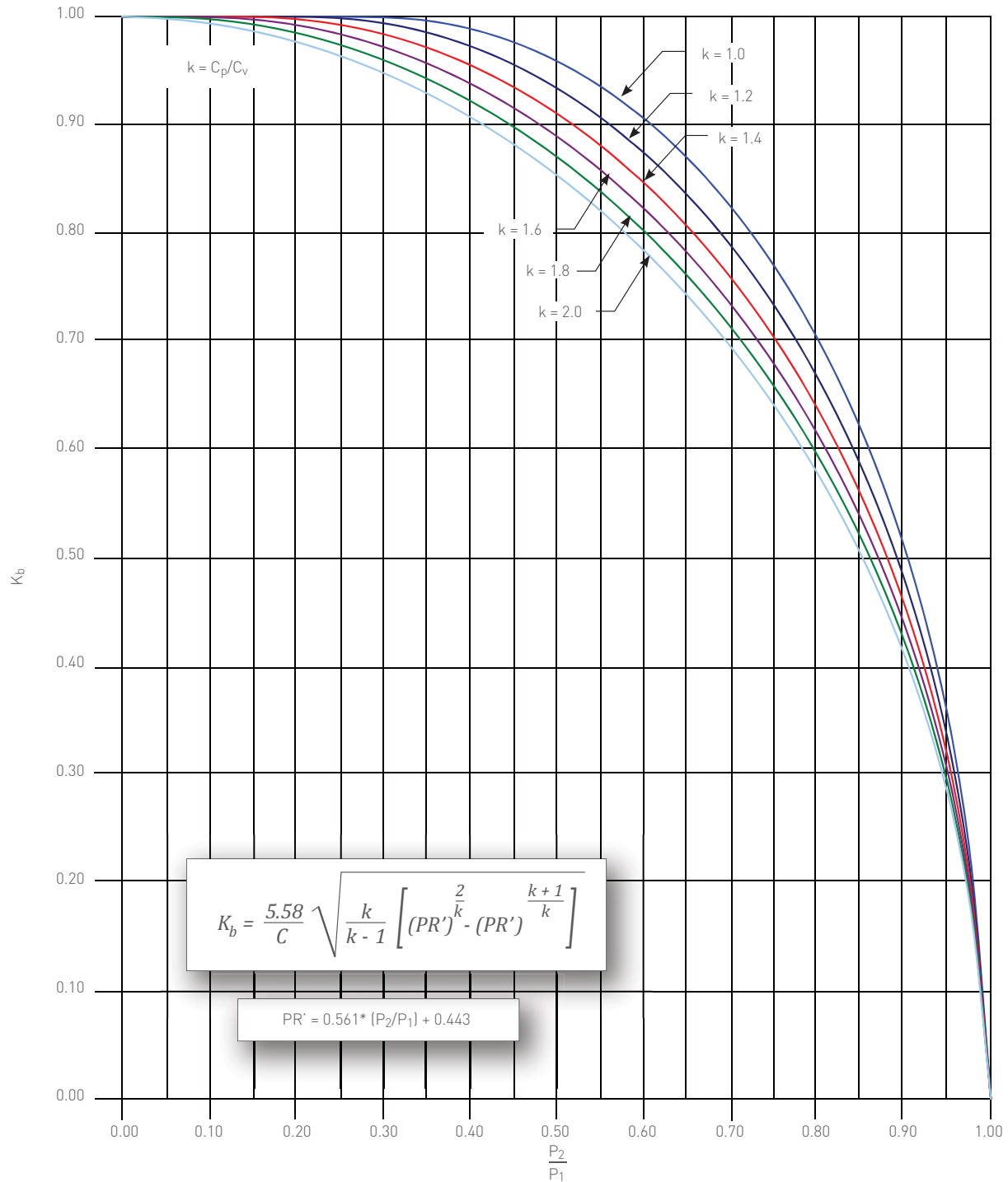
FIGURE 8-8 Crosby Series J0S-E Conventional Direct Spring PRV Back Pressure Correction Factor ( K_b ) - Gas/Steam Service
