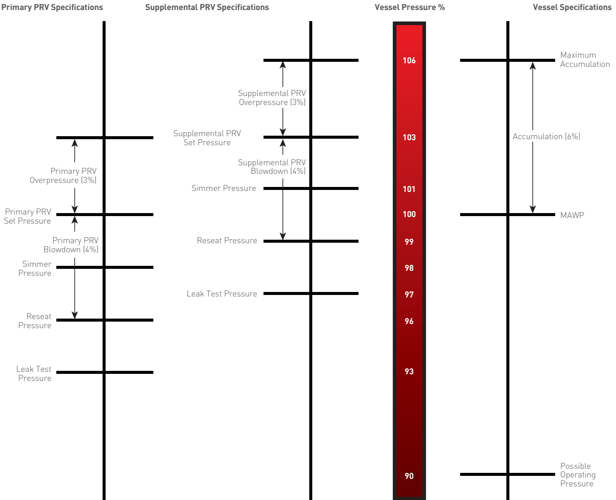
FIGURE 3-2 Typical Section I Multiple PRV Installation
