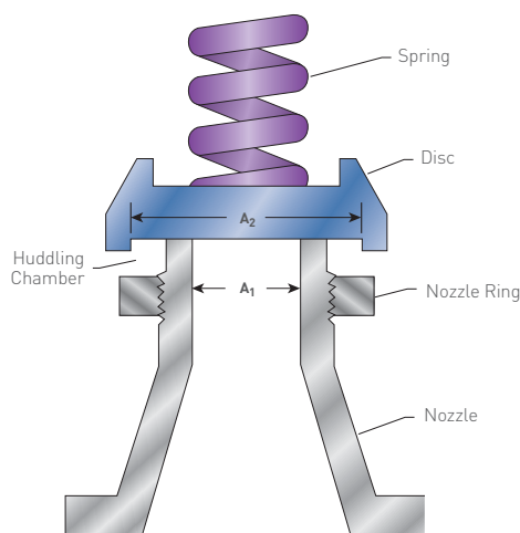
FIGURE 4-5 Generic Direct Spring PRV Trim
