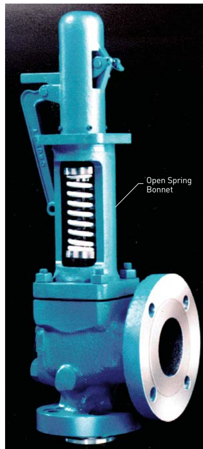
FIGURE 4-15 Open Bonnet Direct Spring PRV
