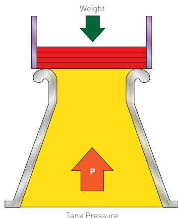
FIGURE 4-1 Weight Loaded Pressure Relief Valve
