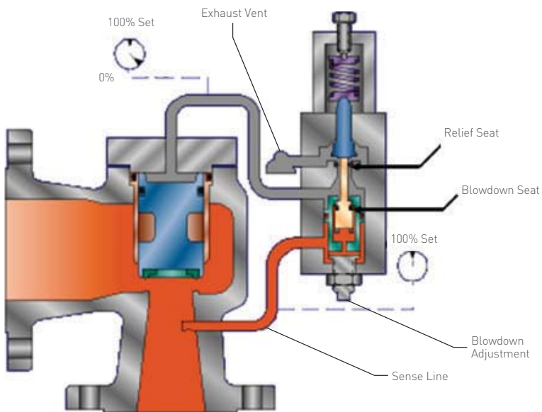
FIGURE 4-29 Pop Action Pilot Operated PRV (open)
