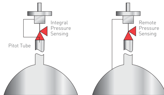
FIGURE 4-36 Remote Sense Pilot Operated PRV
