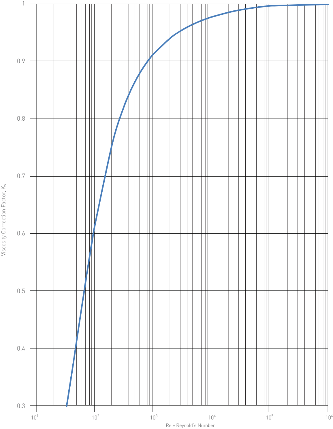
FIGURE 7-29 Viscosity Correction Factor ( K_v )
