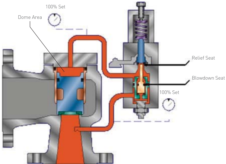
FIGURE 4-28 Pop Action Pilot Operated PRV (closed)
