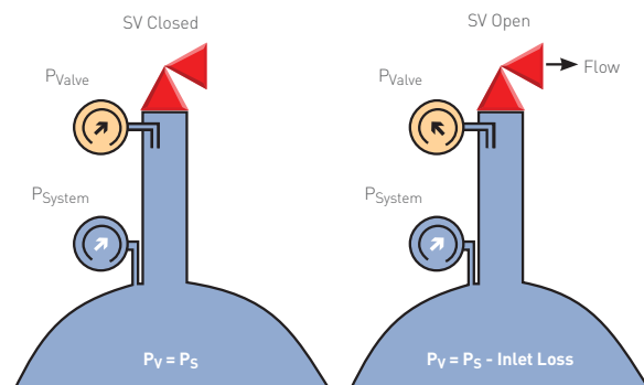
FIGURE 4-18 Inlet Piping Effects on Direct Acting PRV
