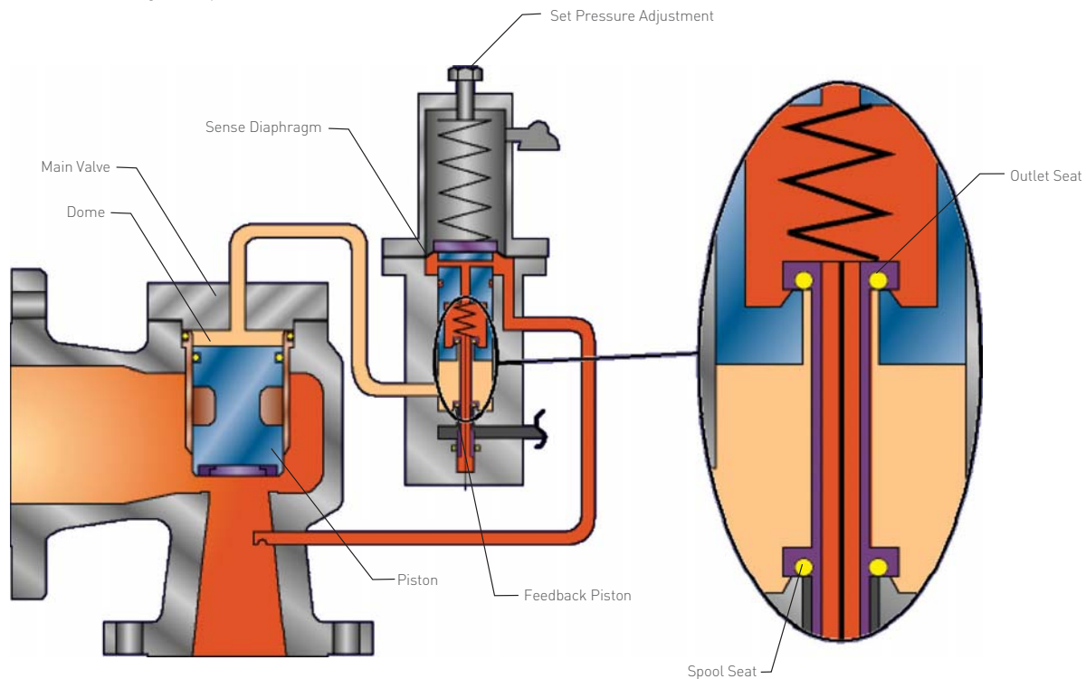
FIGURE 4-37 Balanced Modulating Pilot Operated PRV
