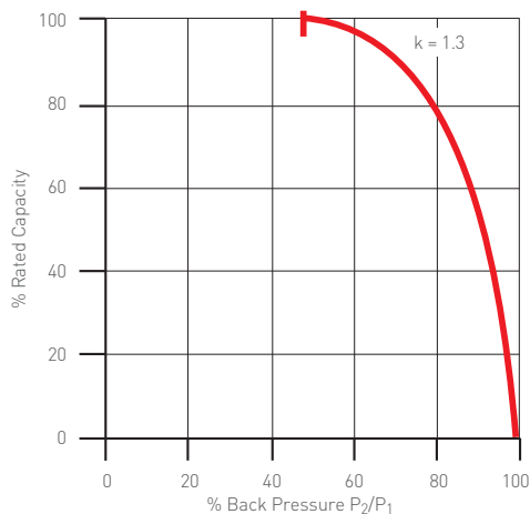
FIGURE 4-38 Sonic to Subsonic Flow Transition
