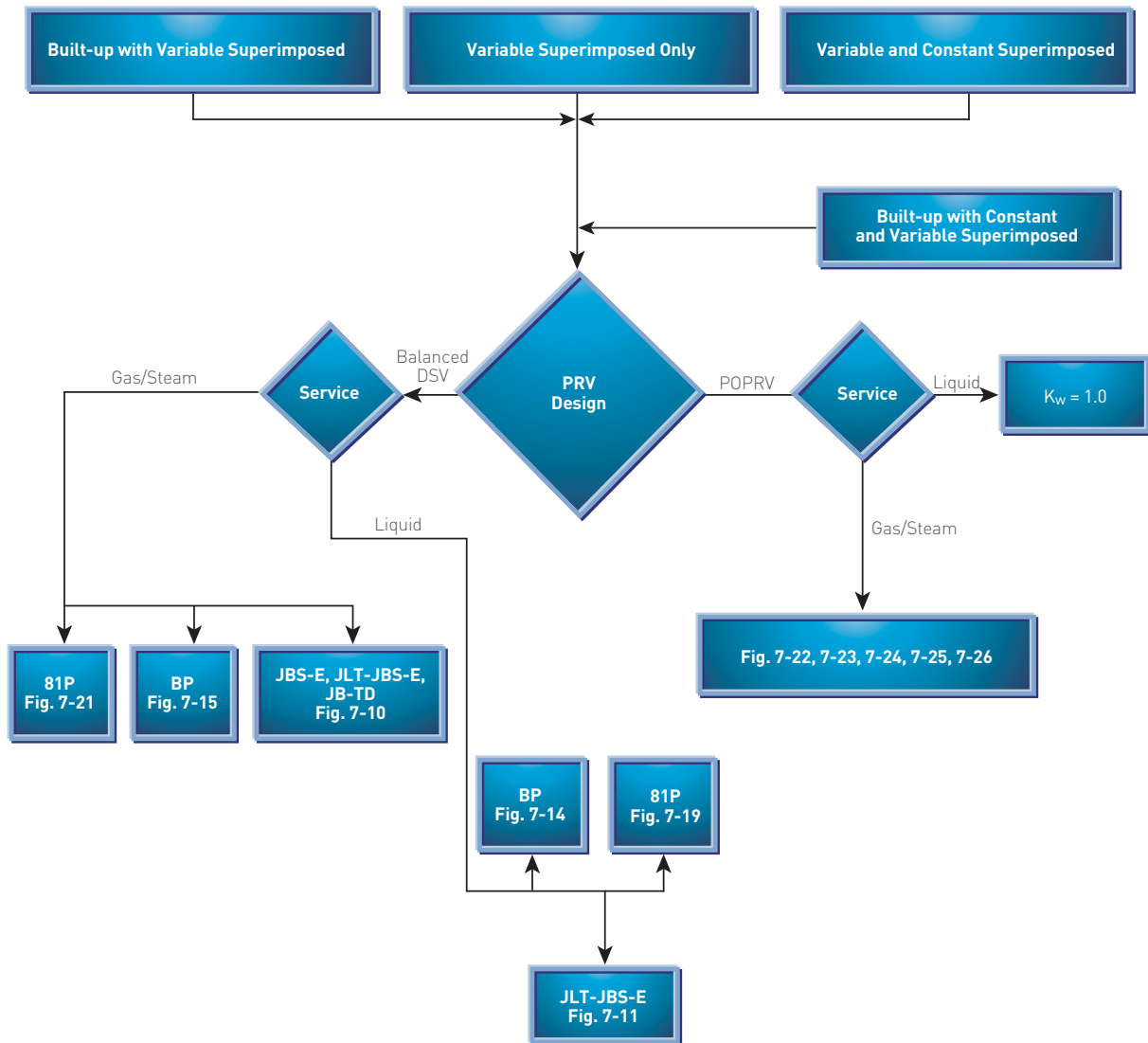
FIGURE 7-6 Valve Selection Recommendations for Variable Superimposed Back Pressure Installations
