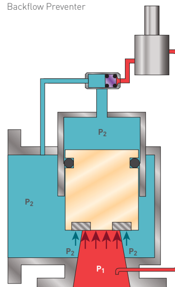
FIGURE 4-40 Backflow Preventer
