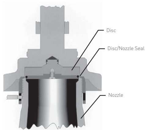
FIGURE 4-13 Metal Seated Direct Spring PRV
