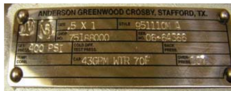
FIGURE 3-12 Typical ASME Section VIII Nameplate
