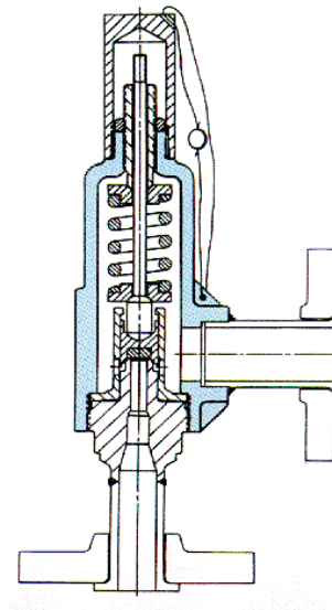
FIGURE 4-18 Inlet Piping Effects on Direct Acting PRV
