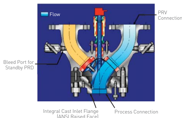
FIGURE 3-5 Safety Selector Valve
