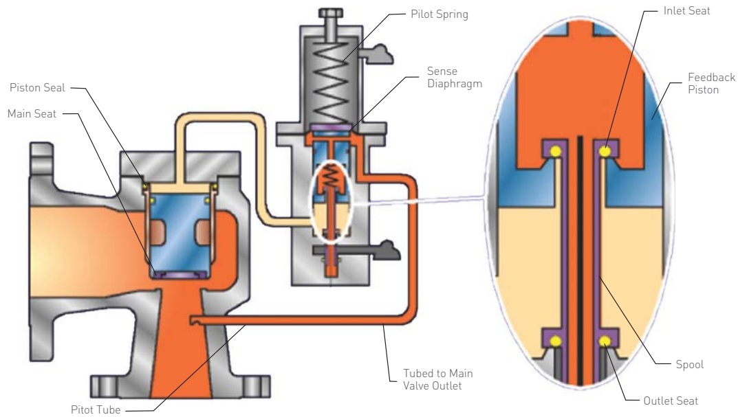
FIGURE 4-32 Modulating Action Pilot Operated PRV (open)
