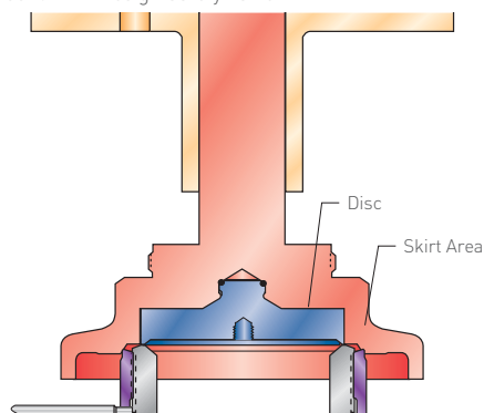
FIGURE 4-6 Section VIII Design Safety Valve Trim
