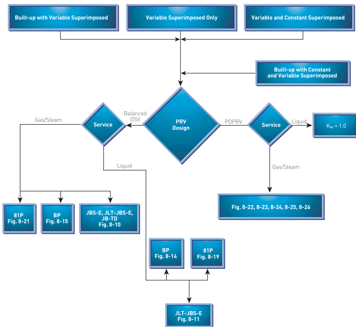
FIGURE 8-6 Valve Selection Recommendations for Variable Superimposed Back Pressure Installations
