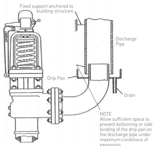
FIGURE 3-6 Recommended ASME Section I Piping Arrangement
