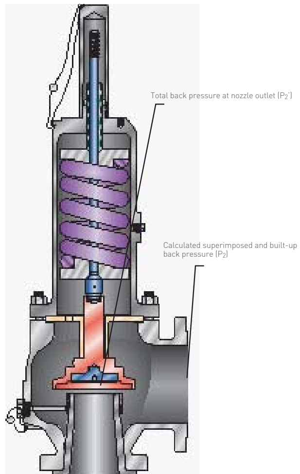
FIGURE 7-3 Relationship of P_2' and P_2
