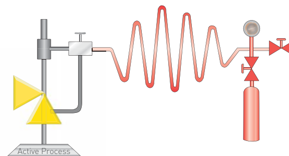
FIGURE 3-4 Pilot Operated PRV Field Test Assembly
