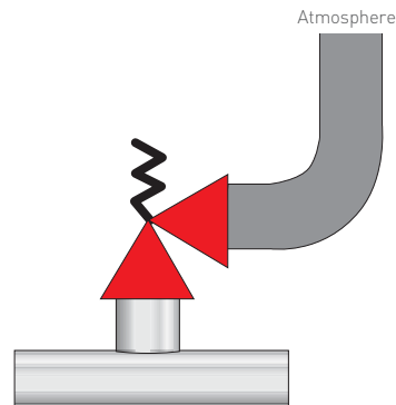
FIGURE 4-19 Tailpipe Discharge Piping
