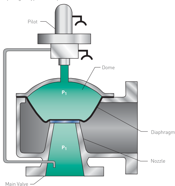
FIGURE 4-26 Diaphragm Type Pilot Operated PRV
