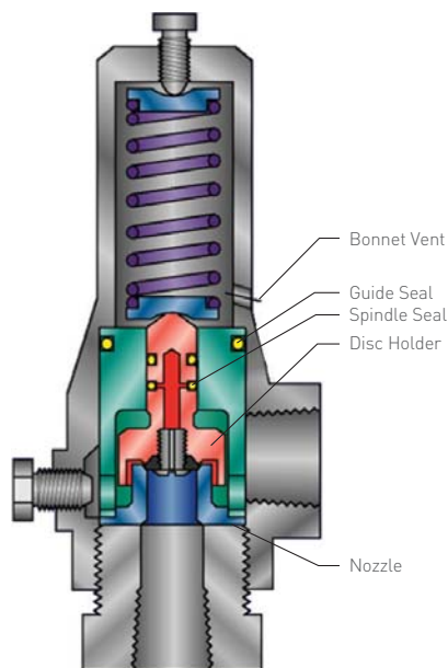
FIGURE 4-24 Balanced Piston Direct Spring PRV
