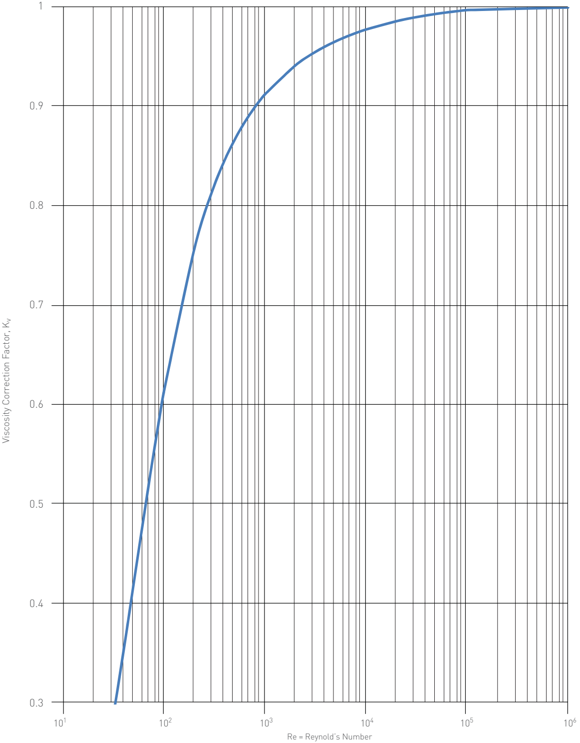
FIGURE 8-29 Viscosity Correction Factor ( K_v )
