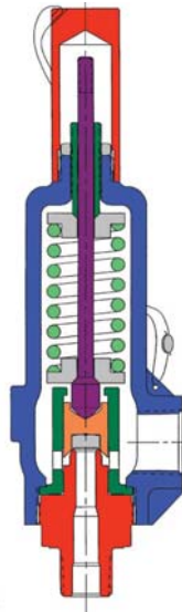
FIGURE 4-18 Inlet Piping Effects on Direct Acting PRV
