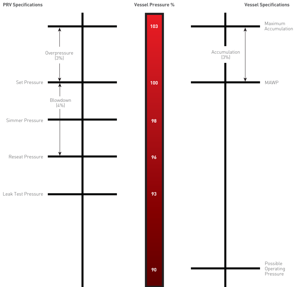
FIGURE 3-1 Typical Section I Single PRV Installation
