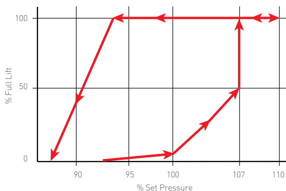
FIGURE 4-12 Typical Relief Valve Lift Characteristic
