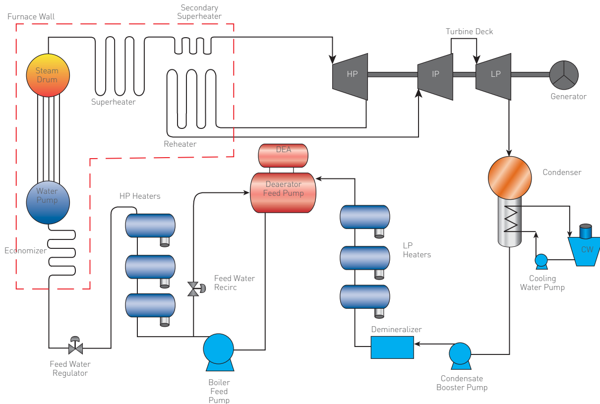
FIGURE 6 - 1 Closed Simple Rankine Steam Cycle
