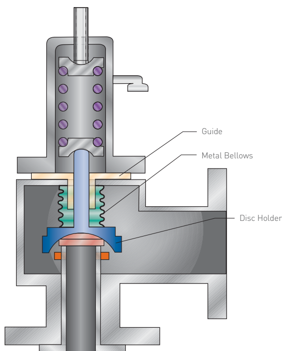
Figure 4-23 Balanced Bellows Direct Spring PRV
