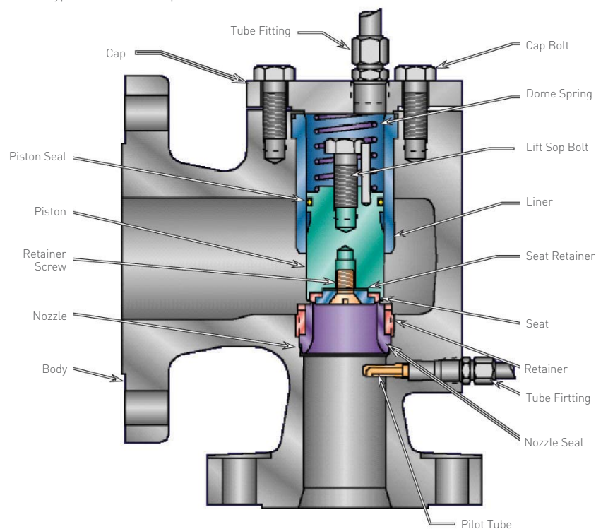
FIGURE 4-35 Piston Type Main Valve Components
