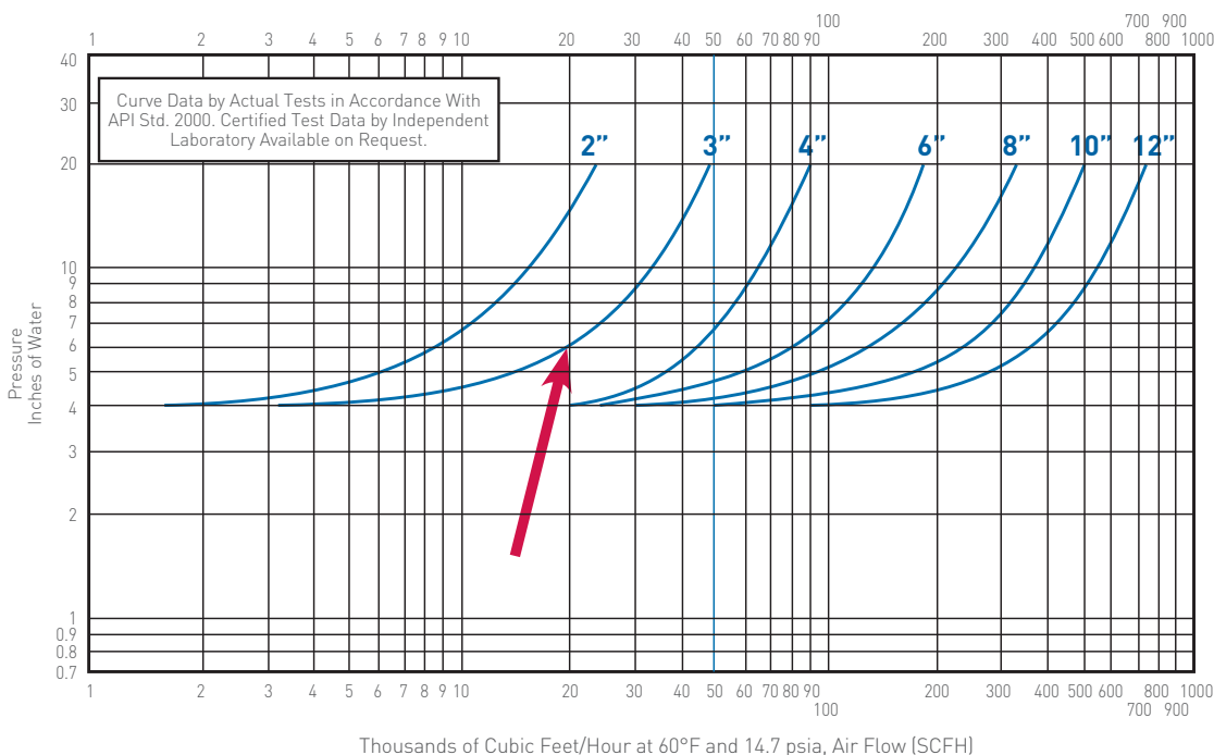
FIGURE 5-1 Varec Brand Pressure Vent Capacity Chart
