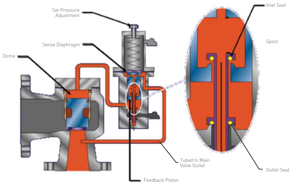
FIGURE 4-31 Modulating Action Pilot Operated PRV (closed)
