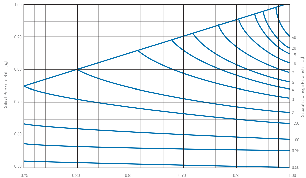
FIGURE 6-3 Saturated Pressure Ratio ( n_c ) Critical Pressure Ratio for Low Subcooled Region Flashing Liquids
