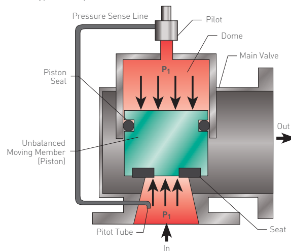
FIGURE 4-25 Piston Type Pilot Operated PRV
