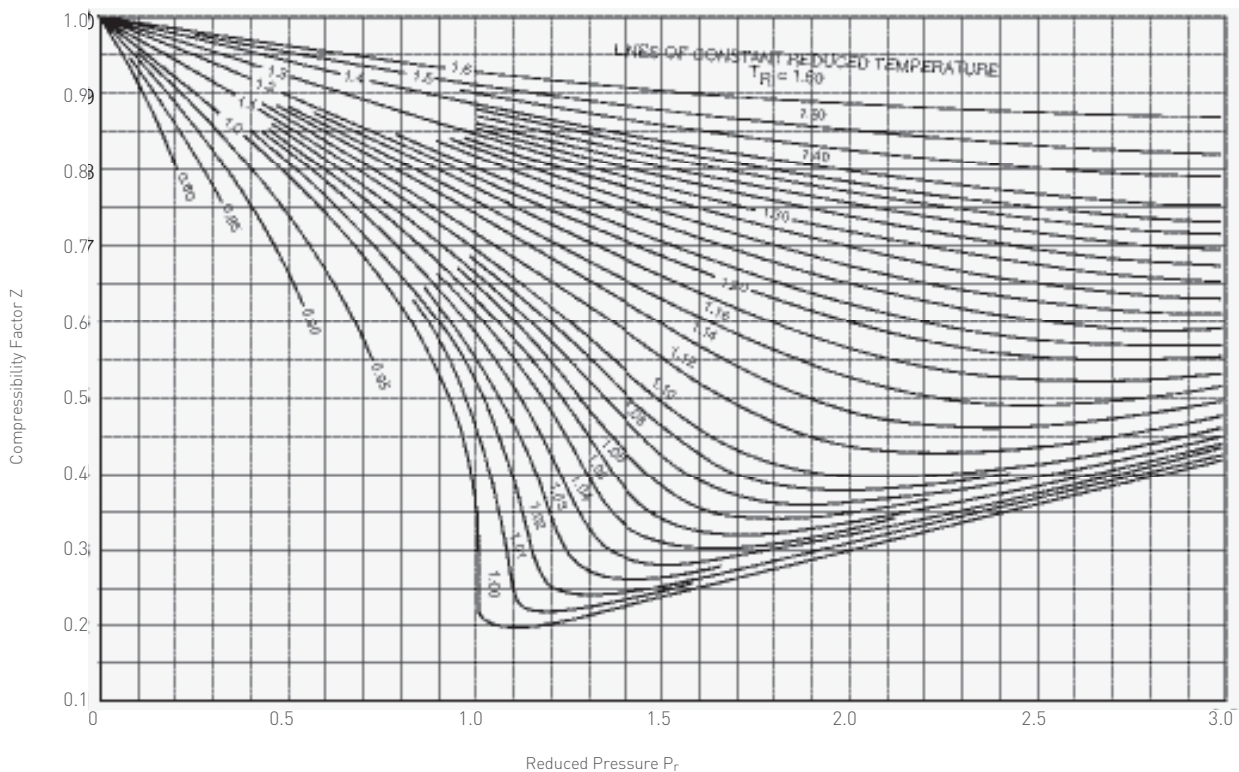
FIGURE 8-1 - Nelson Obert Compressibility Chart
