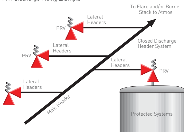
FIGURE 3-14 PRV Discharge Piping Example
