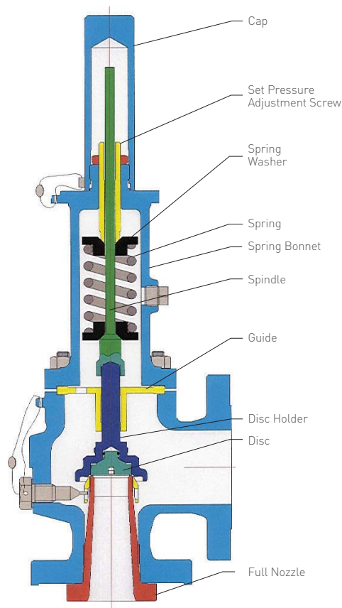
FIGURE 4-14 API 526 Direct Spring PRV
